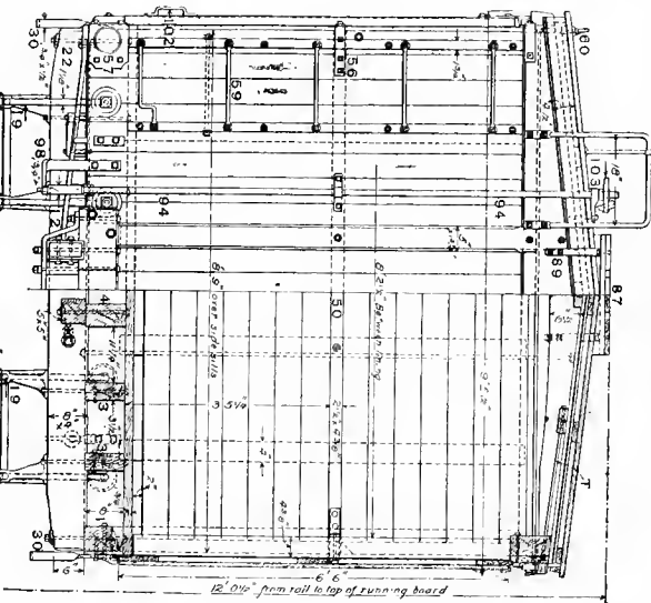
Fig. 244. Part Longitudinal Section and Part Side Elevation.
